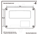
Mounting Template
