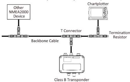
Figure 8 NMEA 2000 Network
