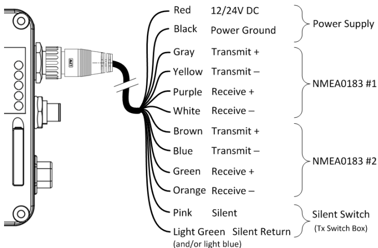
Figure 4 Wiring instructions
