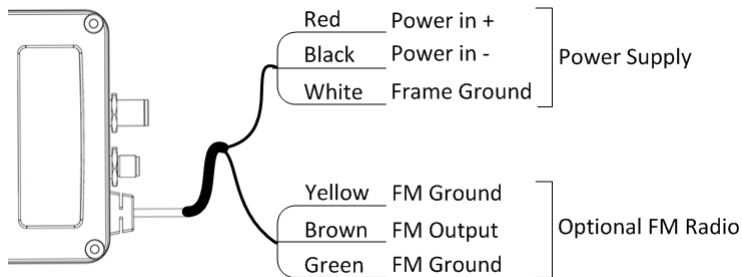
Figure 3 Wiring Instructions
