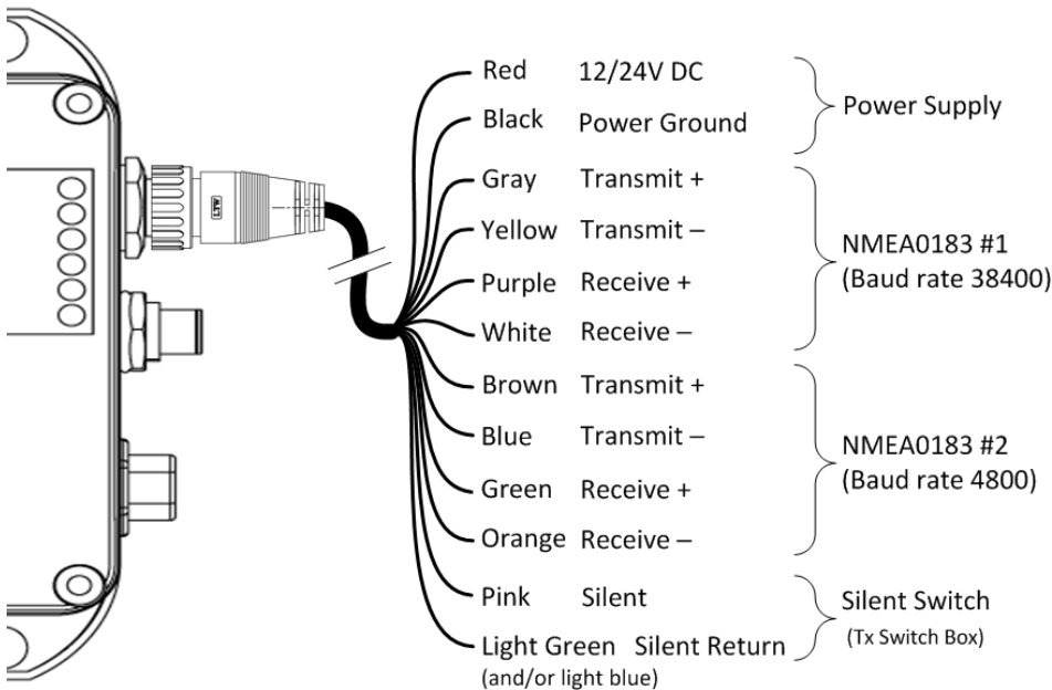
Figure 10 Wiring Instructions
