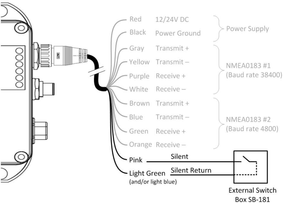
Figure 11 Silent Switch Connection
