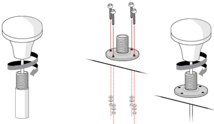
Figure 9 GPS Antenna Mounting
